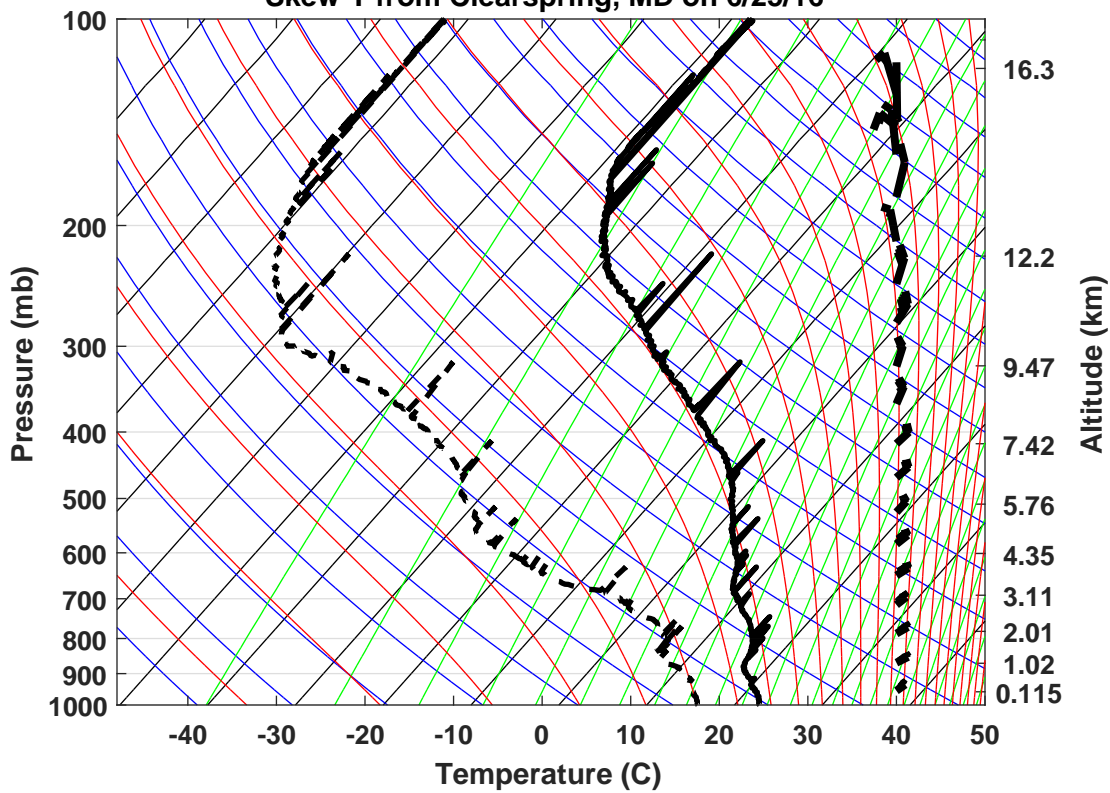
Skew-T from Clearspring, MD on 6/25/16
