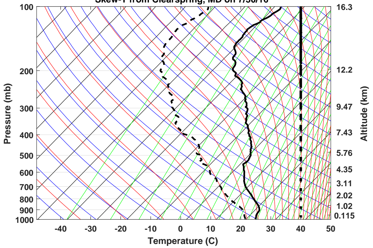
Skew-T from Clearspring, MD on 7/30/16
